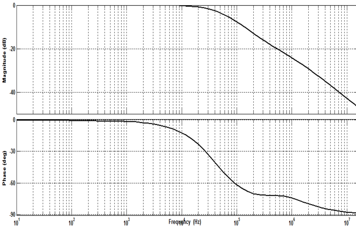
Figure 4. Magnitude and phase of loop-gain
