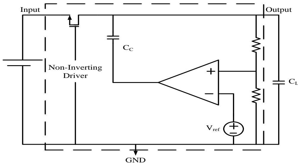
Figure 1. LDO block diagram
