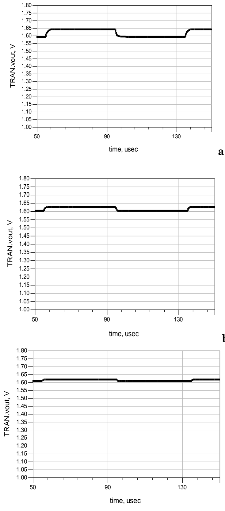
Figure 5. Transient response of the proposed LDO regulator (a)for 0-150 mA load current changes (b)for 0-100 mA load current changes (c)for 0-50 mA load current changes.
