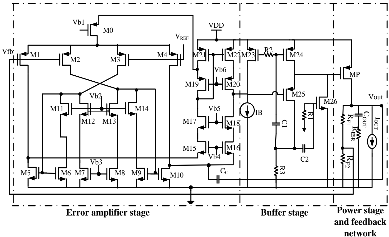
Figure 3. Proposed LDO structure
